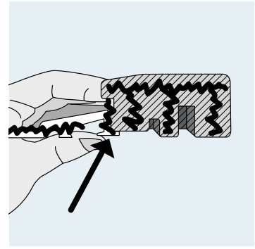
Figure 6: It's important to apply plenty of sealant in the groove
