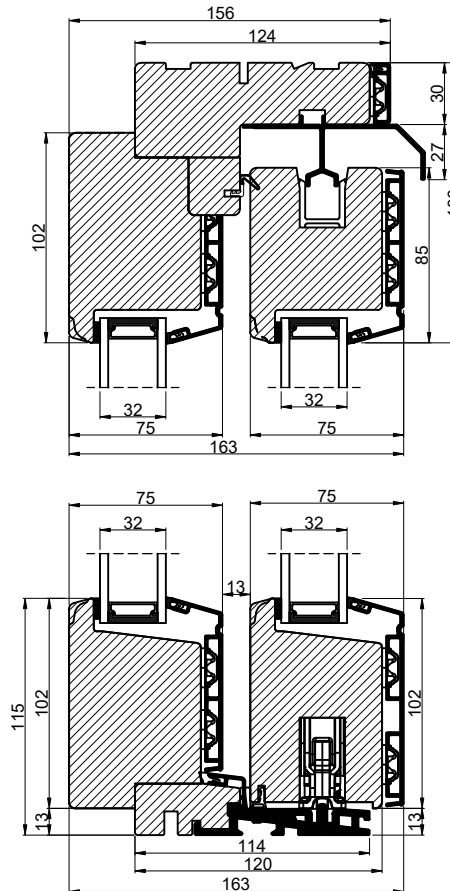
Lodret snit A / Vertical section A
