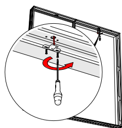
Figur 8: Afmonter softclose-griber
