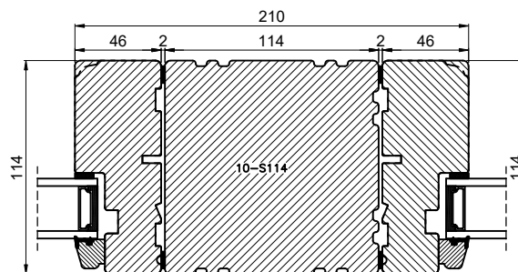
Mellem elementer 180° / Between elements 180°
