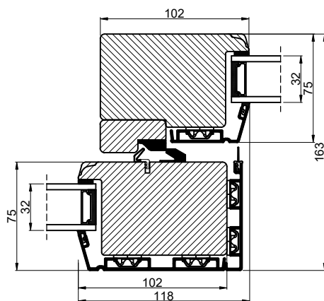
Vandret snit B / Horizontal section B
