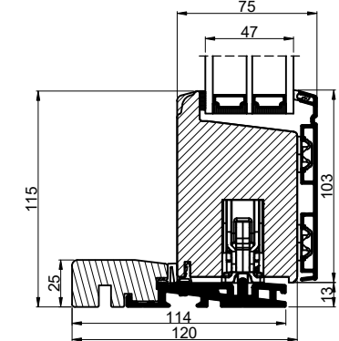
Tilvalg: Fingerskaret egetrin/Optional: Finger-jointed oak threshold
