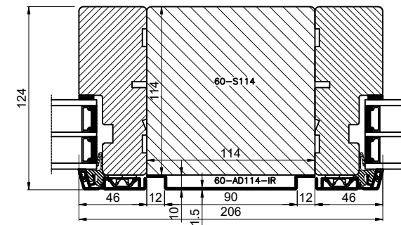
180° corner post
