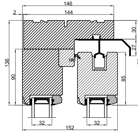
Lodret snit A / Vertical section A
