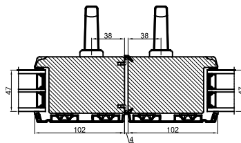
Lodret snit B / Vertical section B
