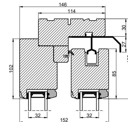
Lodret snit A / Vertical section A
