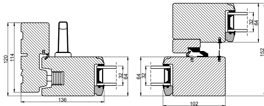
Vandret snit B / Horizontal section B
