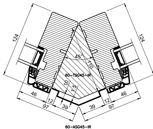
45° corner post
