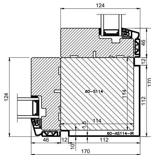
90° corner post
