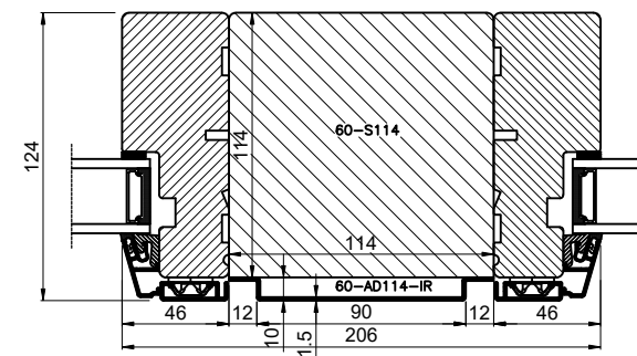
180° corner post
