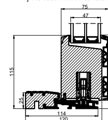
Standard: Malet fyrbund med trinafdækning/ Standard: Painted pine base with threshold covering
