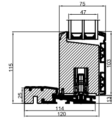
Standard: Malet fyrbund med trinafdækning/ Standard: Painted pine base with threshold covering
