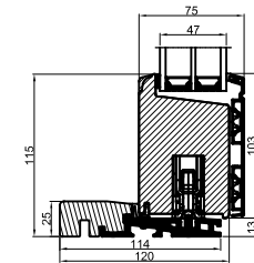
Tilvalg: Fingerskaret egetrin/Optional: Finger-jointed oak threshold
