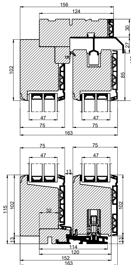
Lodret snit A / Vertical section A
