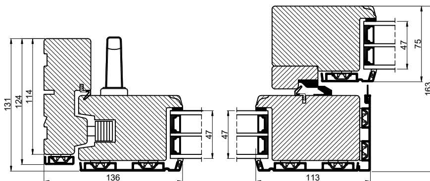
Vandret snit B / Horizontal section B
