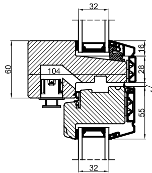
104 mm vandret post
