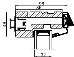
Fast karm, 86 mm karm
