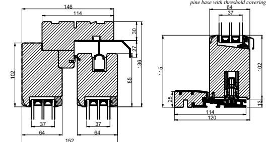
Lodret snit A / Vertical section A
