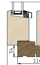
2 Lodret snit i bundkarm/rammer
