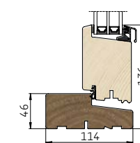
3 Lodret snit i bundkarm/ramme
