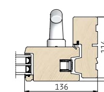
2 Lodret snit i bundkarm/rammer
