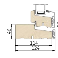
2 Lodret snit i bundkarm/ramme
