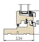
3 Lodret snit i bundkarm/ramme
