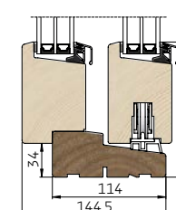
2 Lodret snit i bundkarm/rammer
