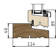
2 Lodret snit i bundkarm/ramme
