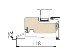
2 Lodret snit i bundkarm/ramme
