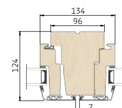
4 Vandret snit i midtkarm/rammer
