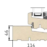
2 Lodret snit i bundkarm/ramme
