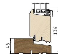
3 Lodret snit i bundkarm/ramme
