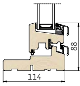
2 Lodret snit i bundkarm/ramme
