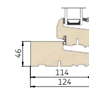
3 Lodret snit i bundkarm/ramme
