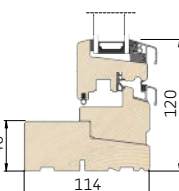
2 Lodret snit i bundkarm/ramme
