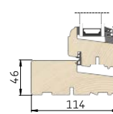
3 Lodret snit i bundkarm/ramme
