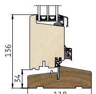
2 Lodret snit i bundkarm/ramme
