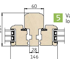
3 Lodret snit i bundkarm/ramme
