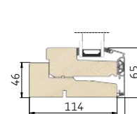
3 Lodret snit i bundkarm/ramme
