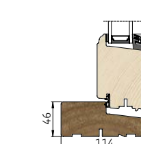
3 Lodret snit i bundkarm/ramme
